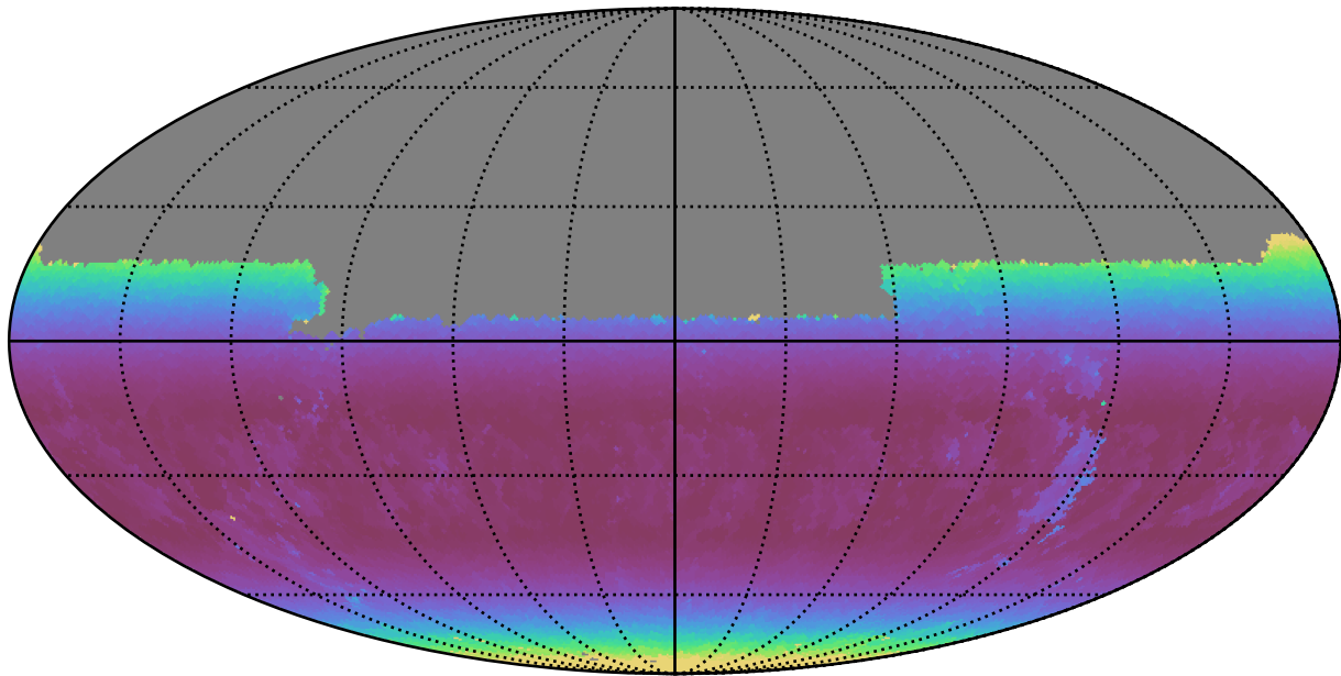
weather_cloudso0v3.4_10yrs Yr 1 y band: Min airmass
