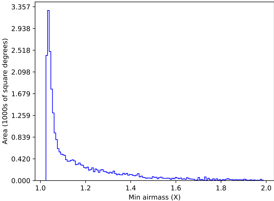
weather_cloudso0v3.4_10yrs Yr 1 i band: Min airmass
