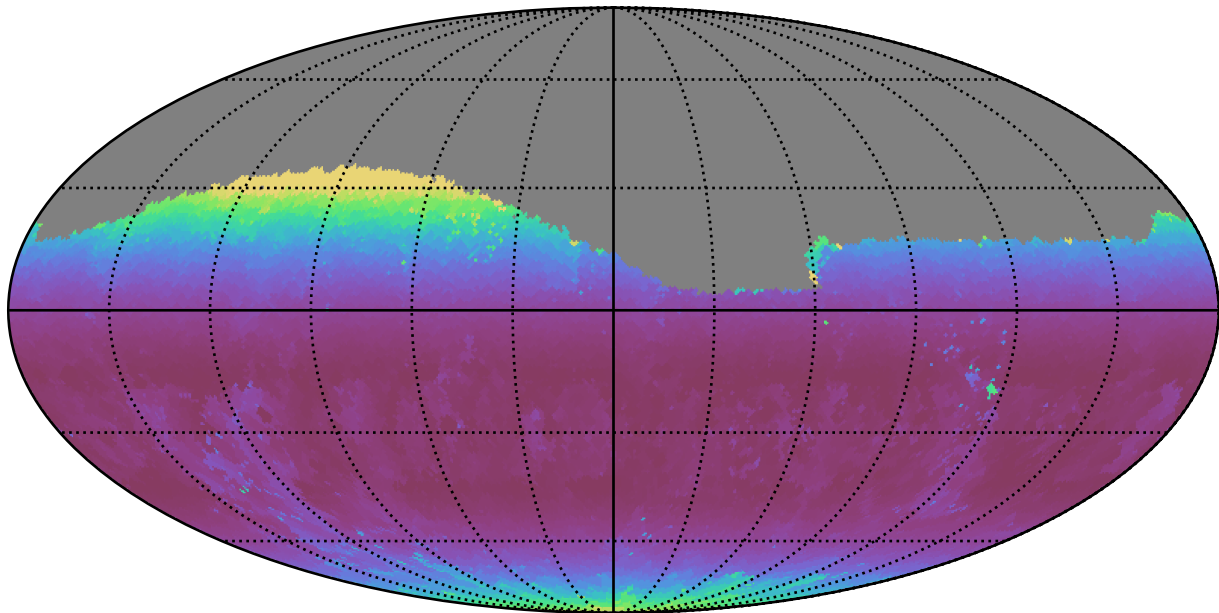
weather_cloudso0v3.4_10yrs Yr 1 g band: Min airmass
