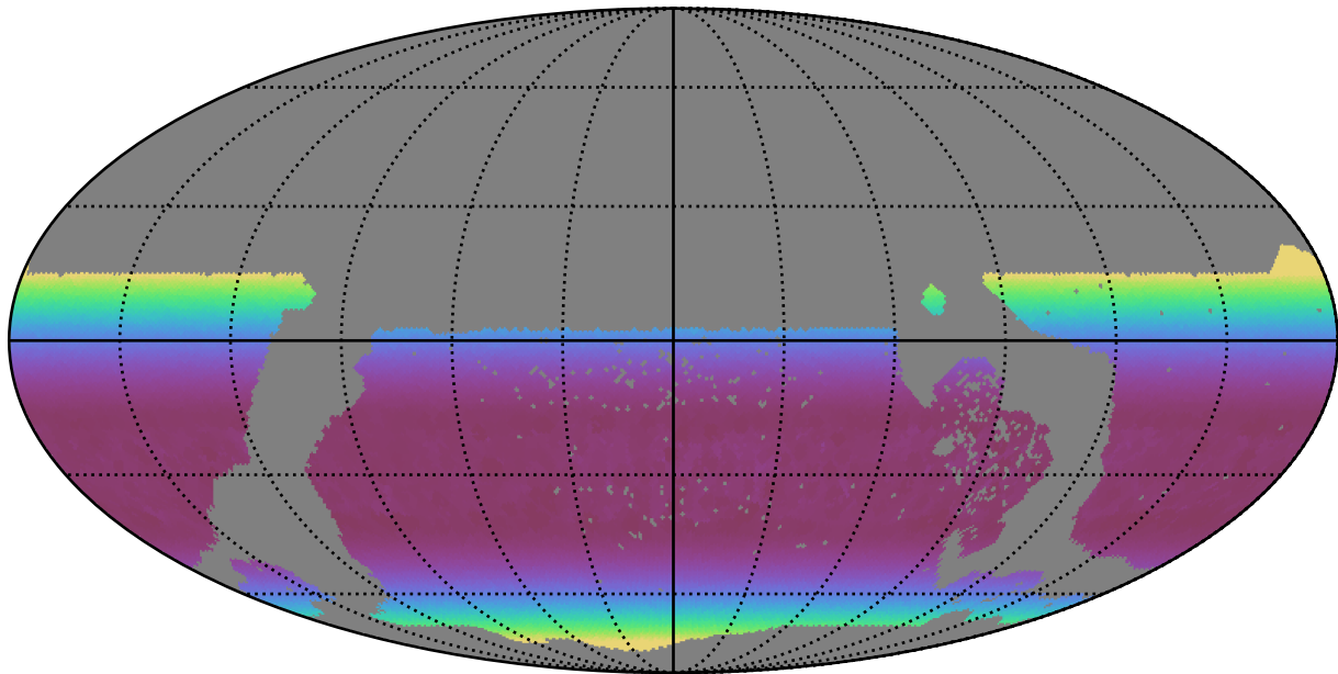
weather_cloudso0v3.4_10yrs WFD z band: Min airmass
