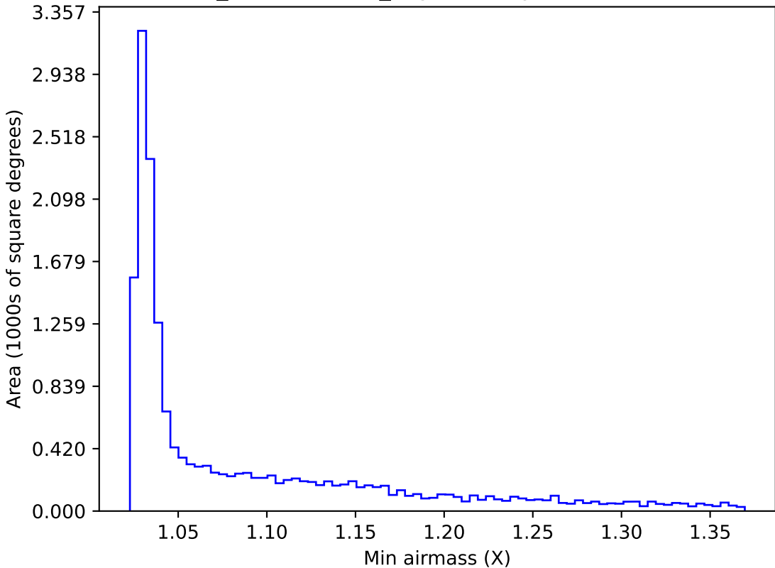
weather_cloudso0v3.4_10yrs WFD y band: Min airmass
