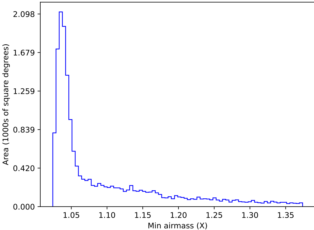
weather_cloudso0v3.4_10yrs WFD u band: Min airmass
