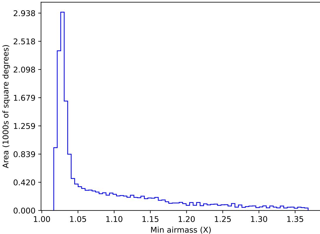
weather_cloudso0v3.4_10yrs WFD r band: Min airmass
