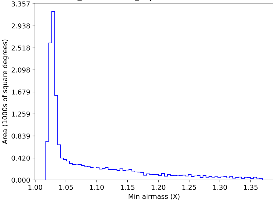
weather_cloudso0v3.4_10yrs WFD i band: Min airmass
