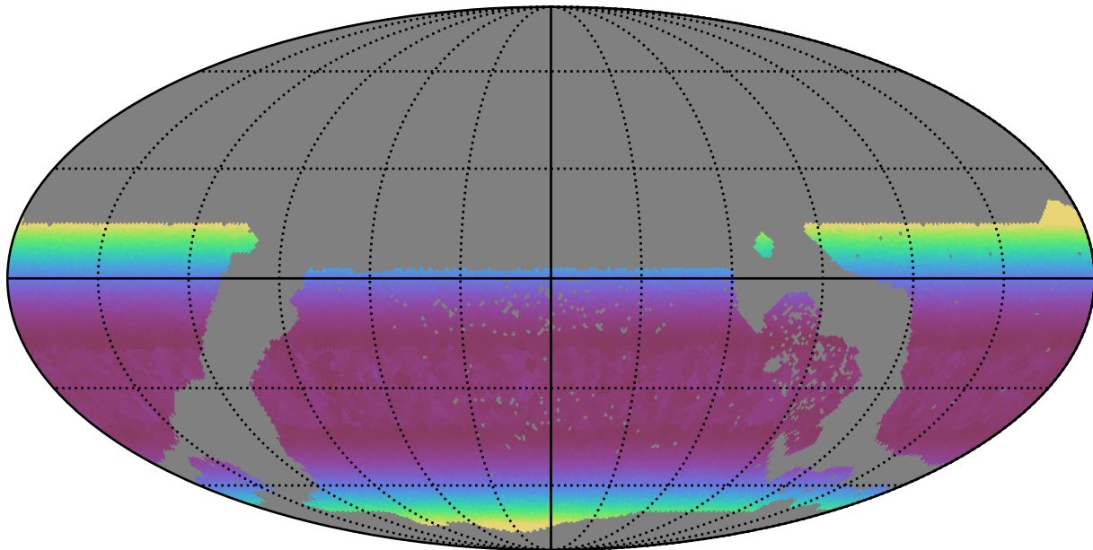
weather_cloudso0v3.4_10yrs WFD g band: Min airmass
