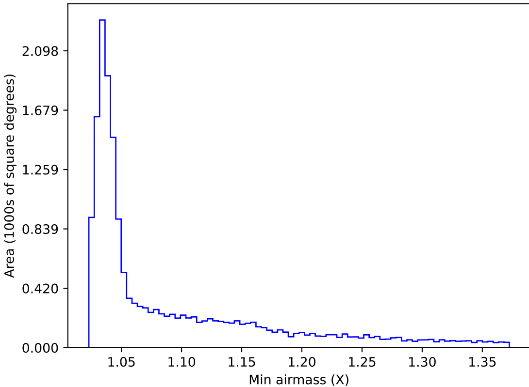
weather_cloudso0v3.4_10yrs WFD g band: Min airmass
