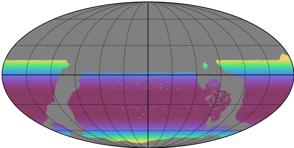
weather_cloudso0v3.4_10yrs WFD all bands: Min airmass
