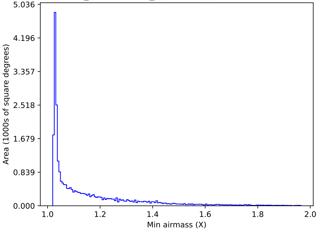
weather_cloudso0v3.4_10yrs All sky z band: Min airmass
