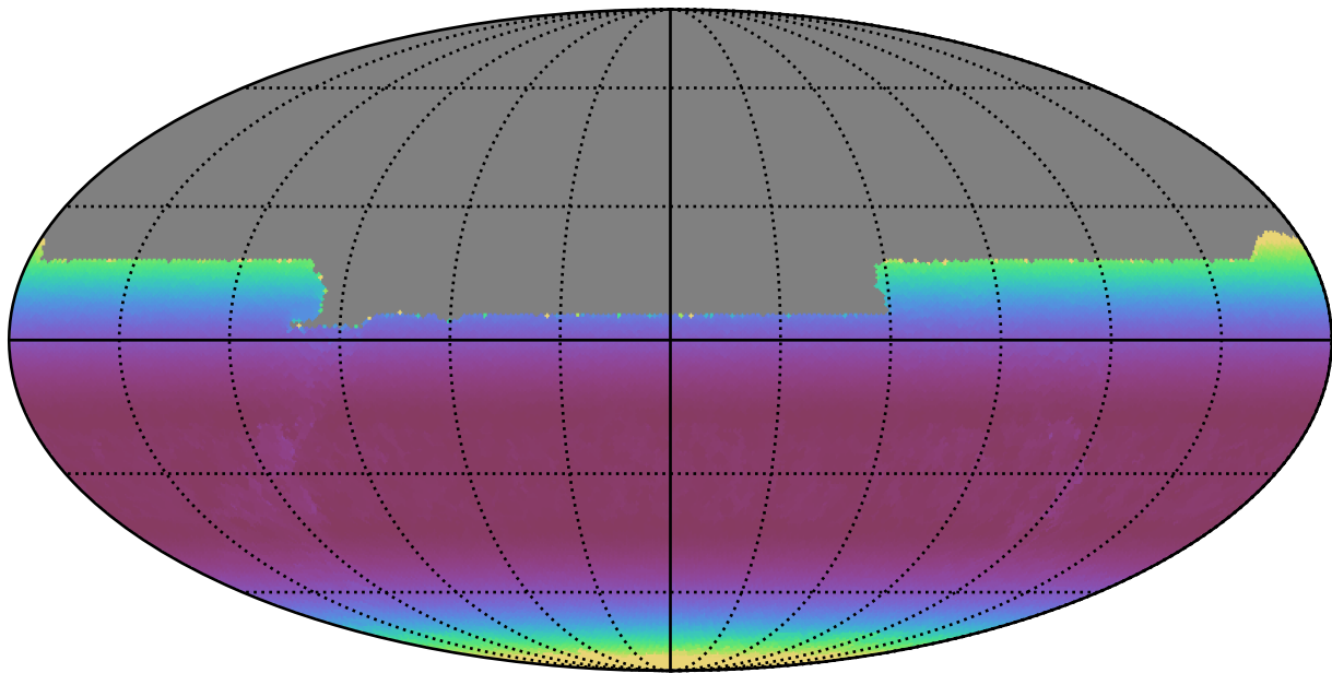
weather_cloudso0v3.4_10yrs All sky y band: Min airmass
