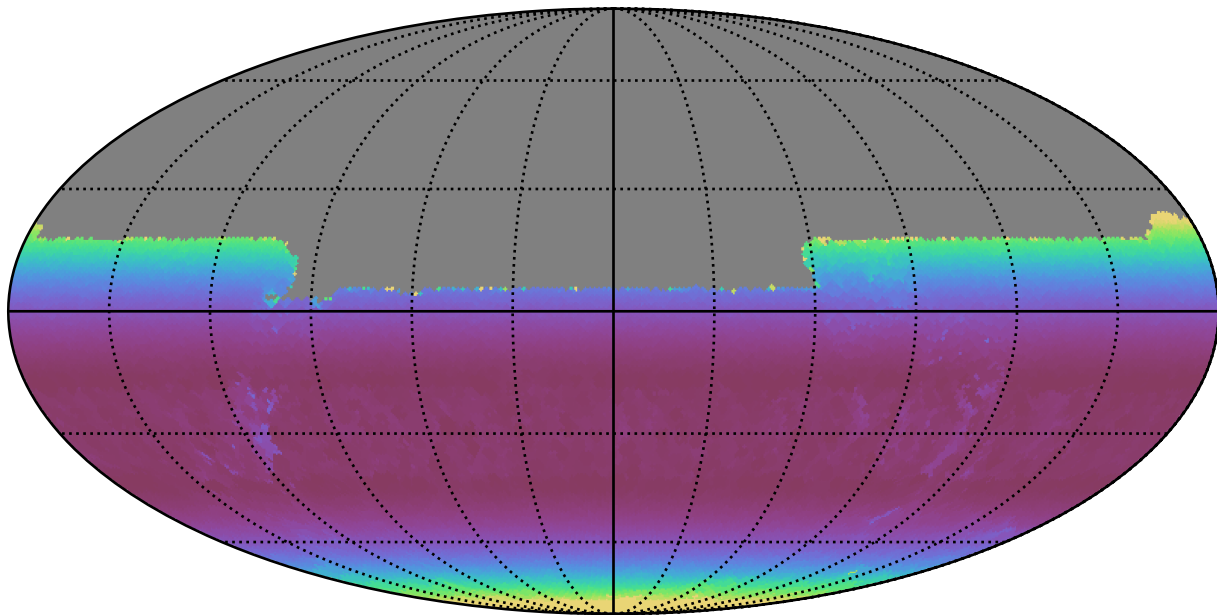
weather_cloudso0v3.4_10yrs All sky u band: Min airmass
