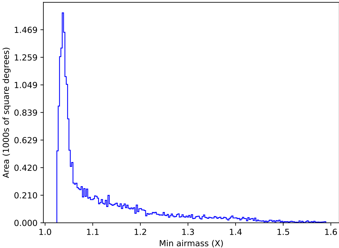
weather_cloudso0v3.4_10yrs All sky u band: Min airmass
