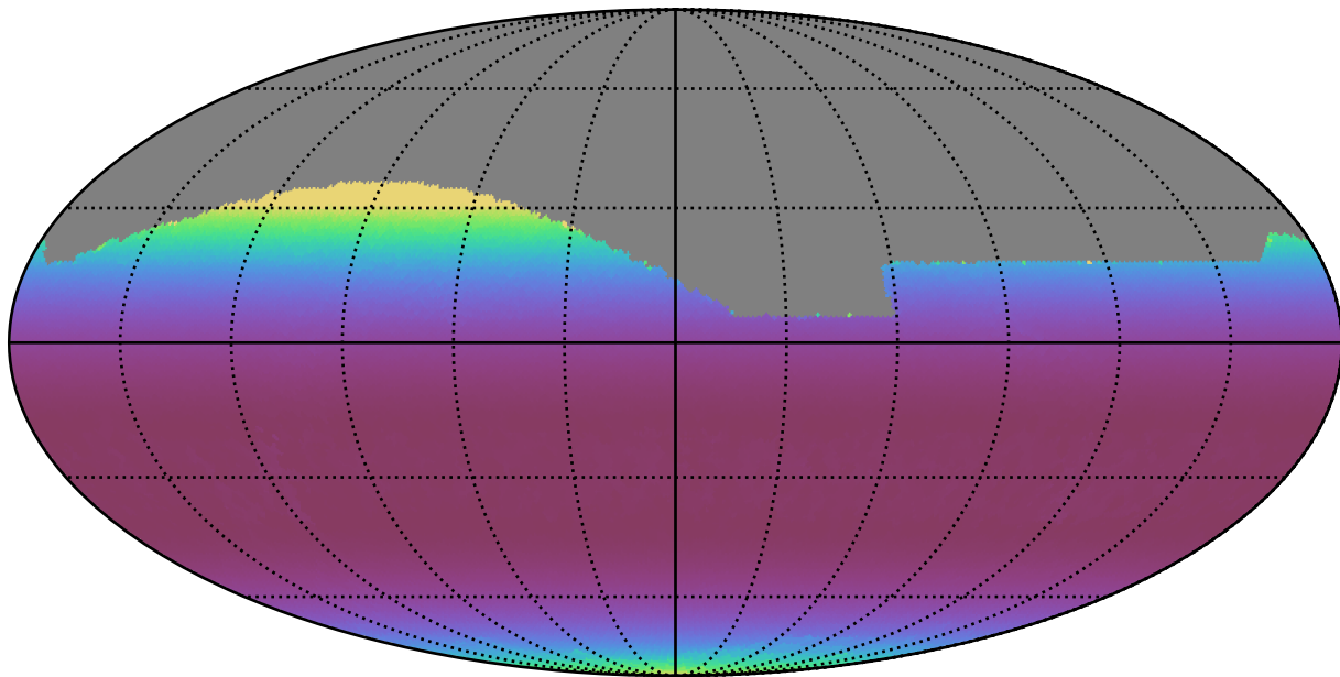
weather_cloudso0v3.4_10yrs All sky r band: Min airmass
