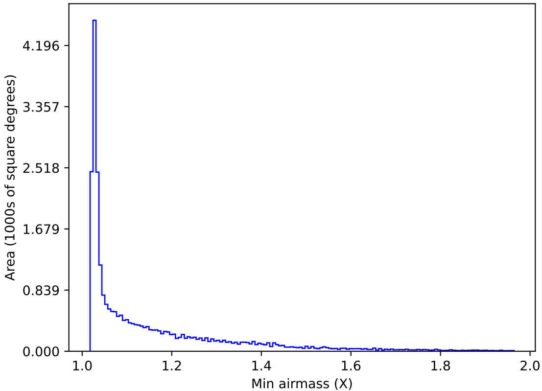
weather_cloudso0v3.4_10yrs All sky r band: Min airmass
