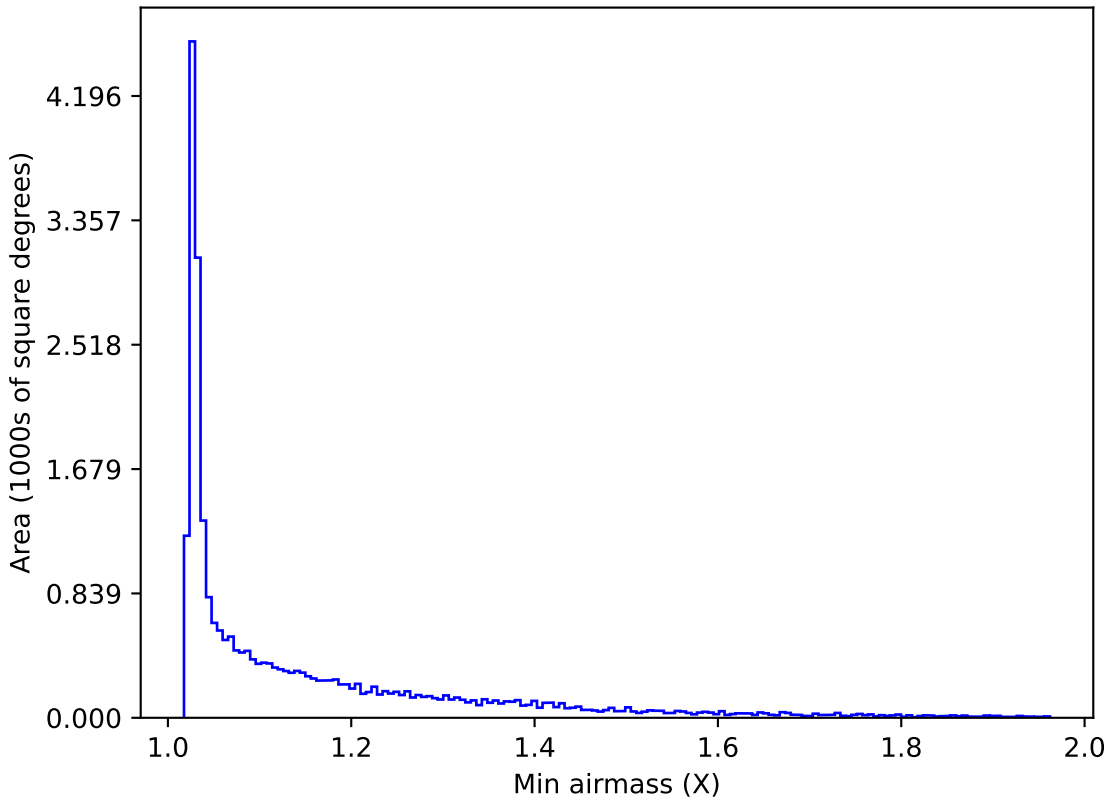
weather_cloudso0v3.4_10yrs All sky i band: Min airmass
