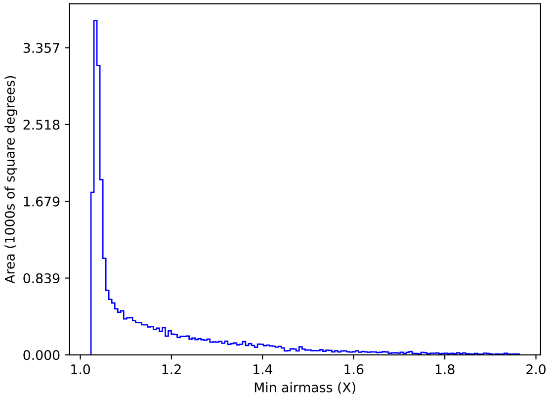
weather_cloudso0v3.4_10yrs All sky g band: Min airmass
