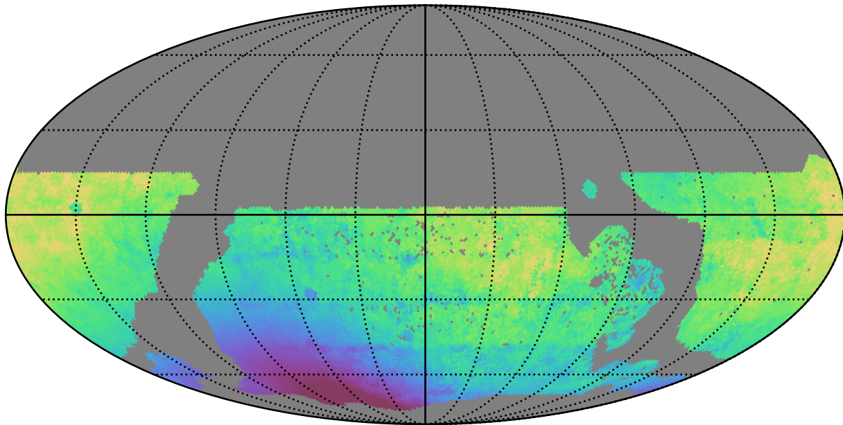
weather_cloudso0v3.4_10yrs WFD z band: Median solarElong
