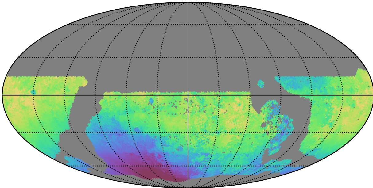
weather_cloudso0v3.4_10yrs WFD u band: Median solarElong
