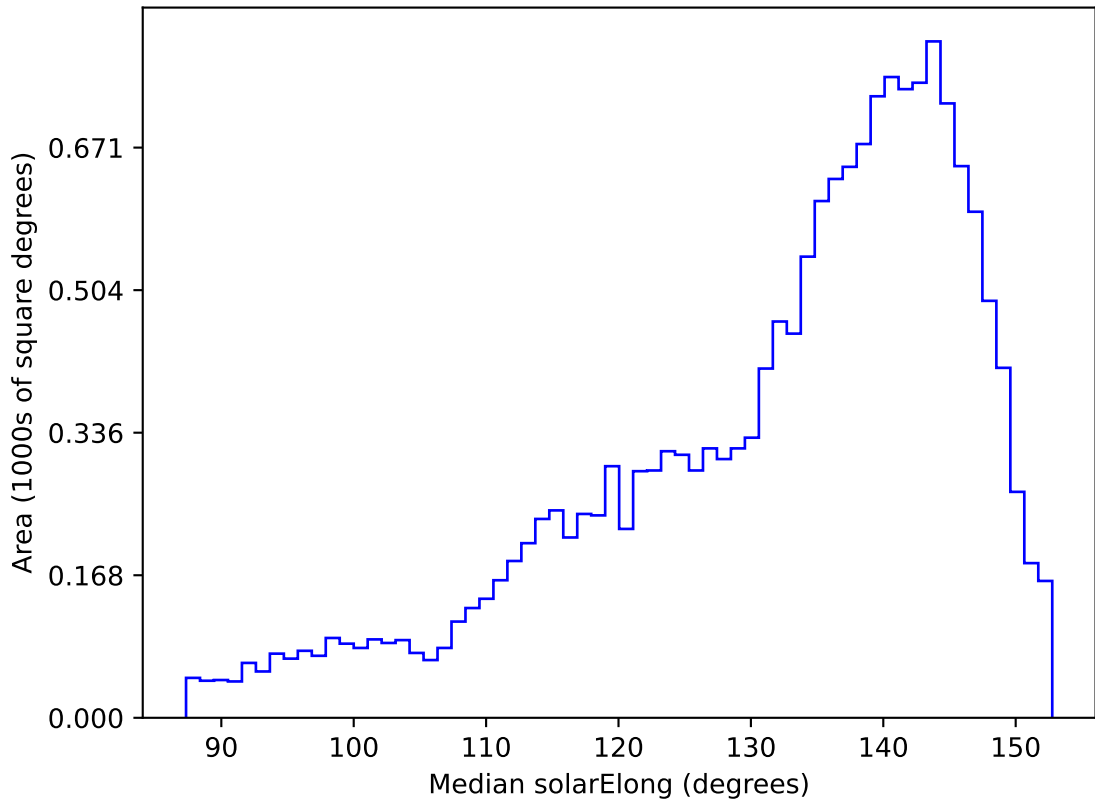
weather_cloudso0v3.4_10yrs WFD u band: Median solarElong
