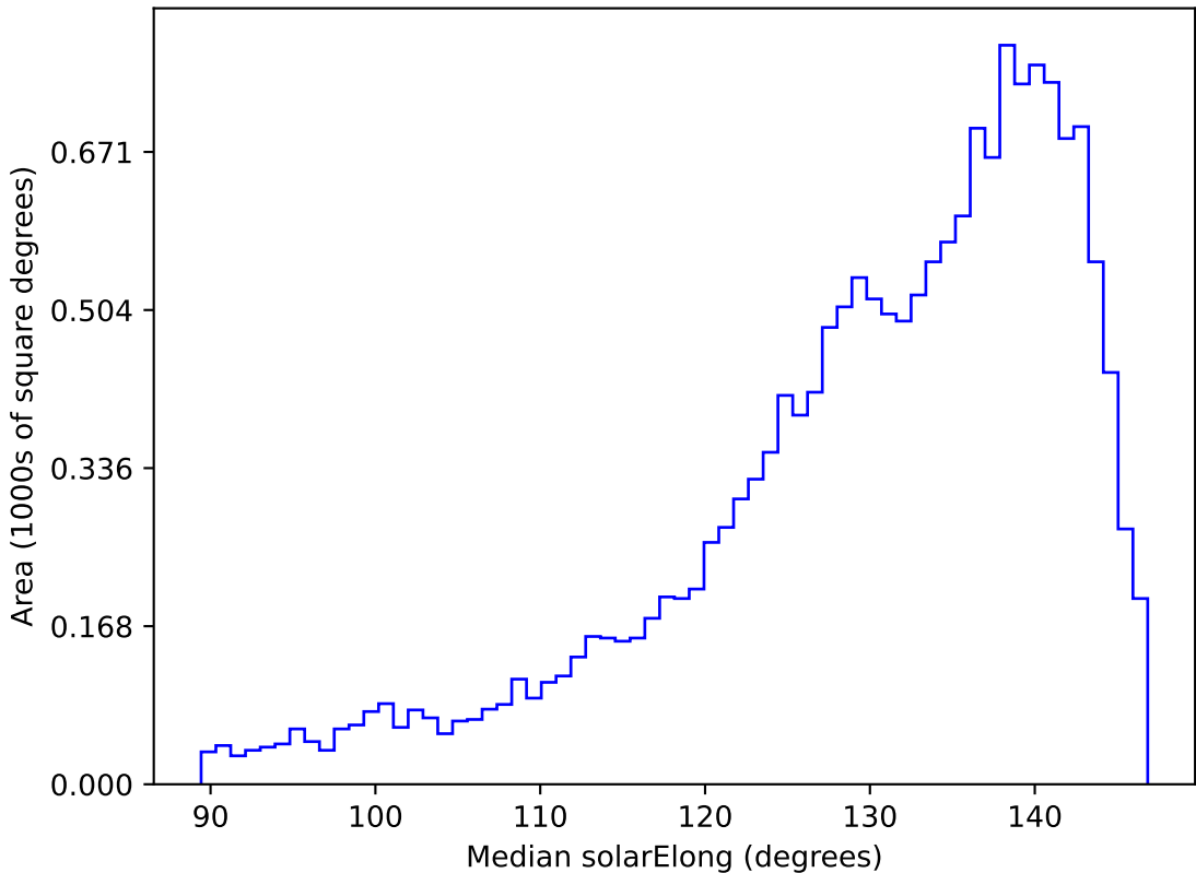
weather_cloudso0v3.4_10yrs WFD r band: Median solarElong
