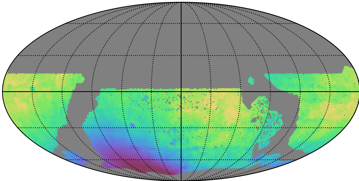
weather_cloudso0v3.4_10yrs WFD i band: Median solarElong
