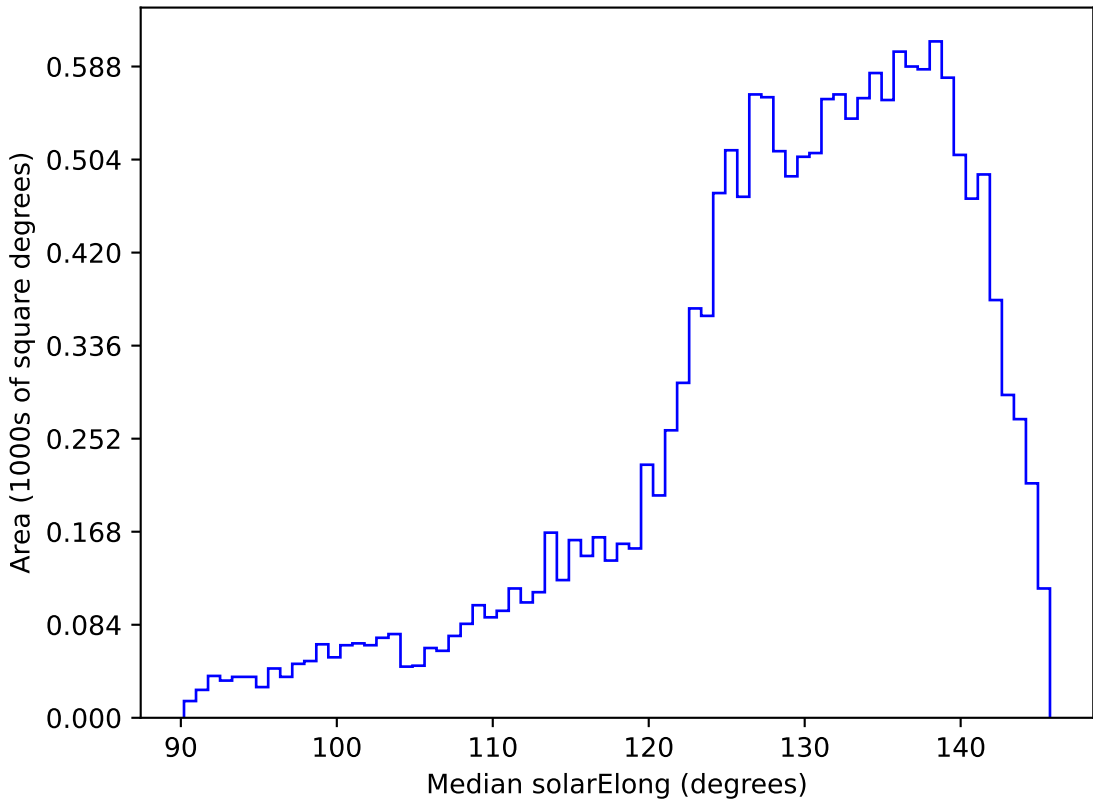
weather_cloudso0v3.4_10yrs WFD i band: Median solarElong
