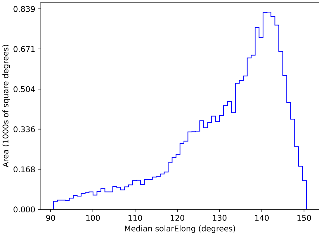
weather_cloudso0v3.4_10yrs WFD g band: Median solarElong
