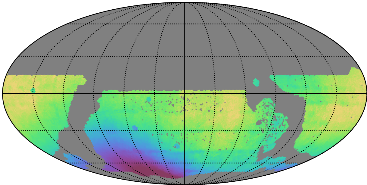
weather_cloudso0v3.4_10yrs WFD all bands: Median solarElong
