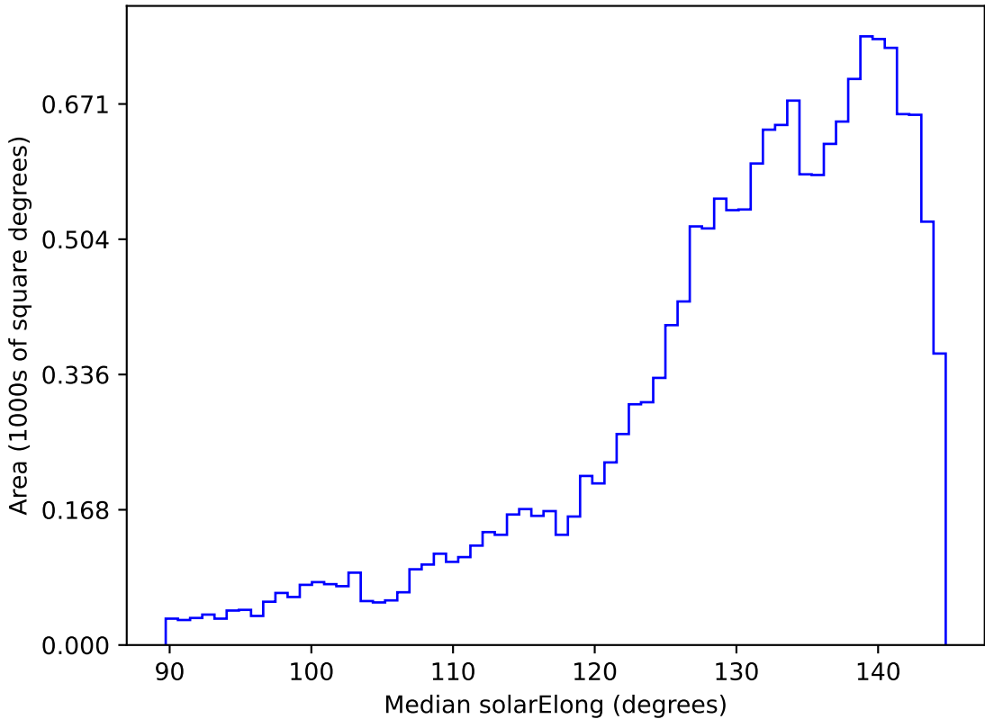
weather_cloudso0v3.4_10yrs WFD all bands: Median solarElong
