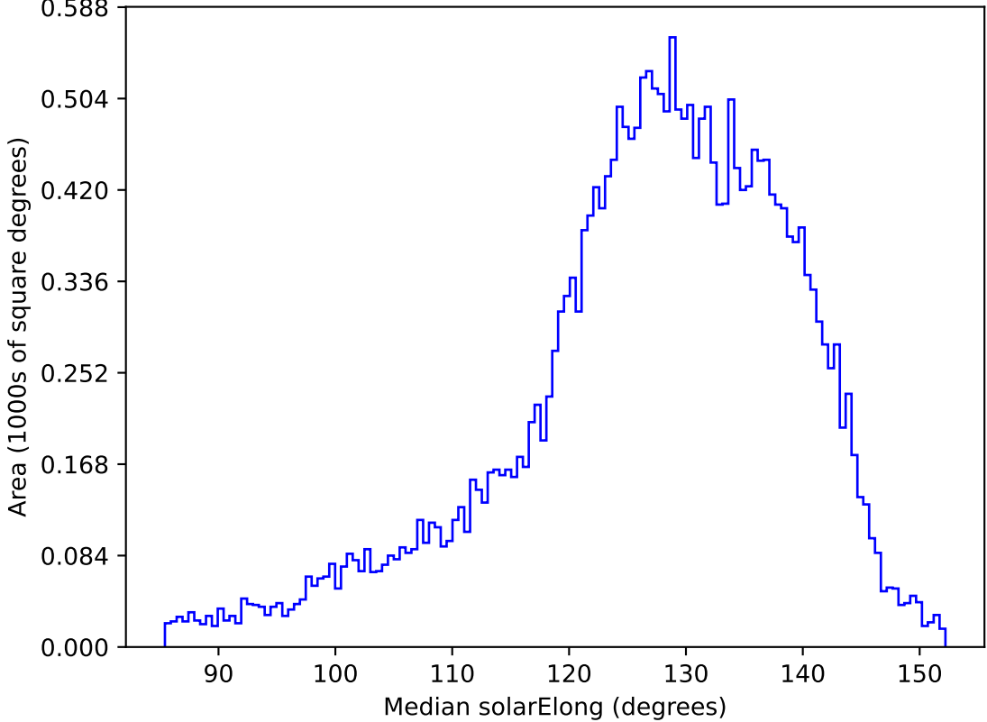
weather_cloudso0v3.4_10yrs All sky z band: Median solarElong
