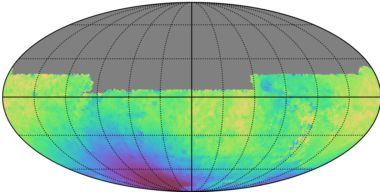
weather_cloudso0v3.4_10yrs All sky y band: Median solarElong
