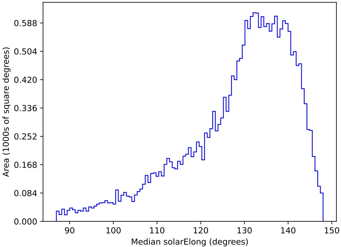
weather_cloudso0v3.4_10yrs All sky y band: Median solarElong
