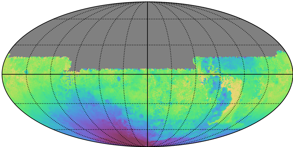
weather_cloudso0v3.4_10yrs All sky u band: Median solarElong
