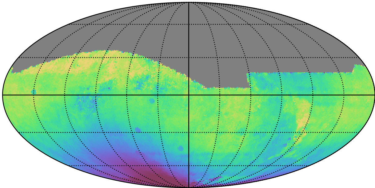
weather_cloudso0v3.4_10yrs All sky r band: Median solarElong
