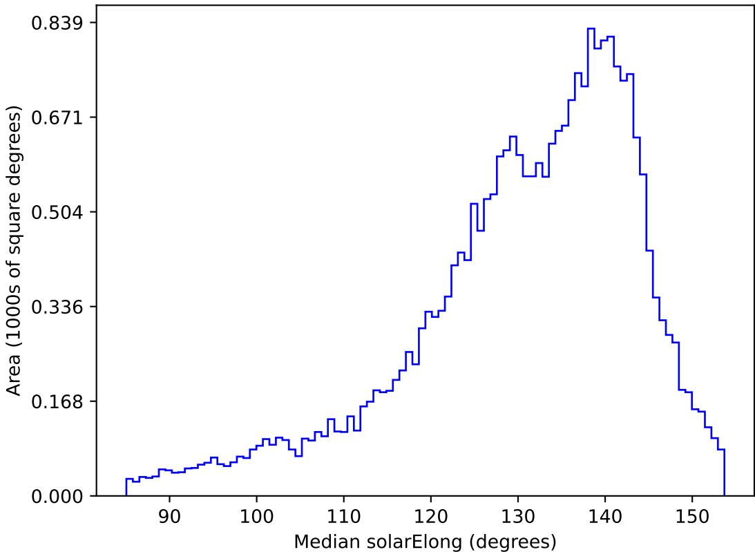
weather_cloudso0v3.4_10yrs All sky r band: Median solarElong
