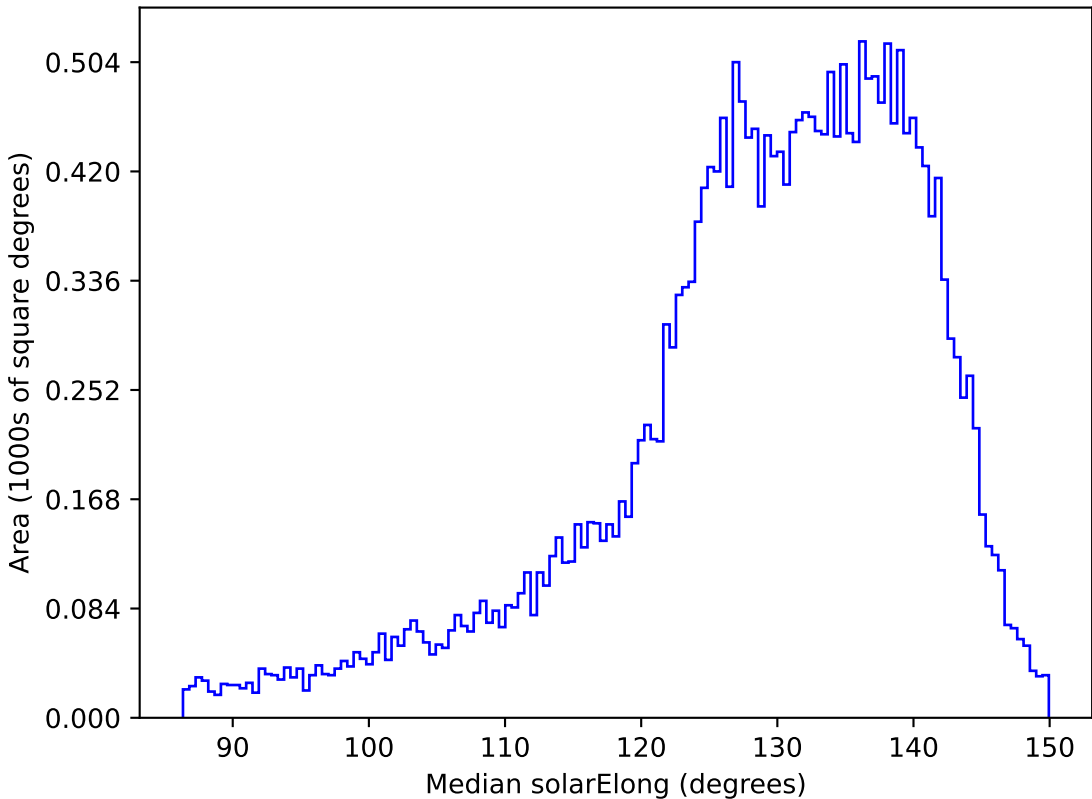
weather_cloudso0v3.4_10yrs All sky i band: Median solarElong
