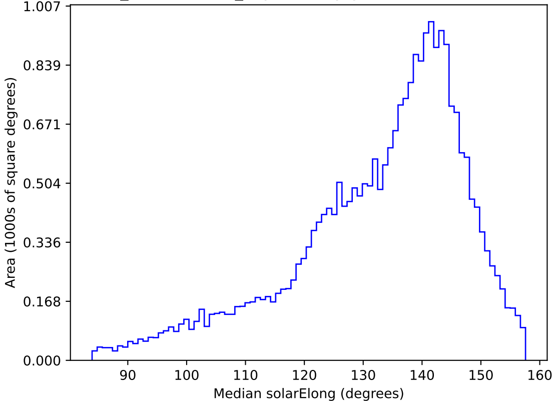
weather_cloudso0v3.4_10yrs All sky g band: Median solarElong
