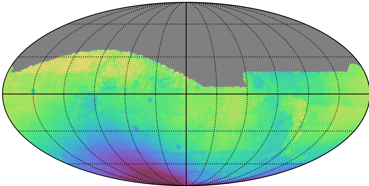
weather_cloudso0v3.4_10yrs All sky all bands: Median solarElong
