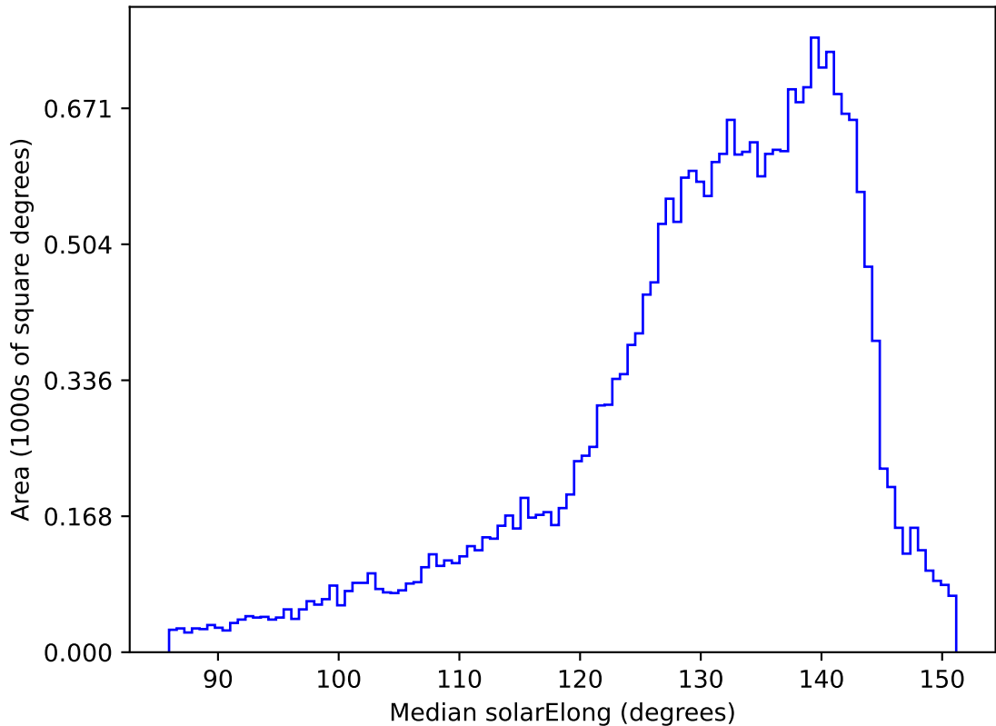
weather_cloudso0v3.4_10yrs All sky all bands: Median solarElong
