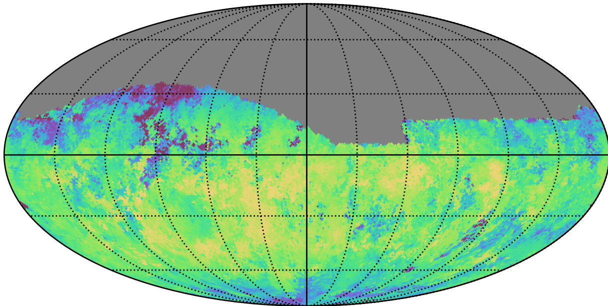
weather_cloudso0v3.4_10yrs Yr 1 z band: Median skyBrightness
