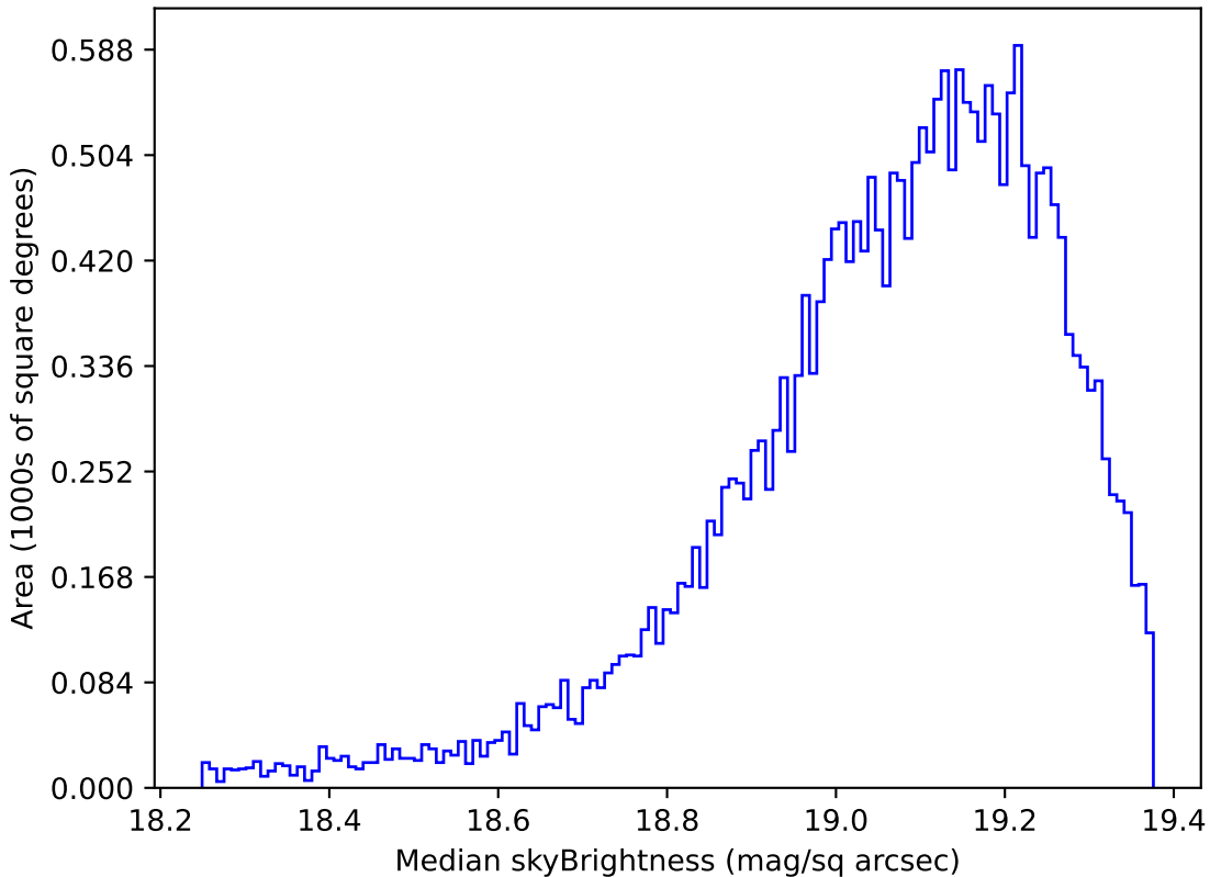
weather_cloudso0v3.4_10yrs Yr 1 z band: Median skyBrightness
