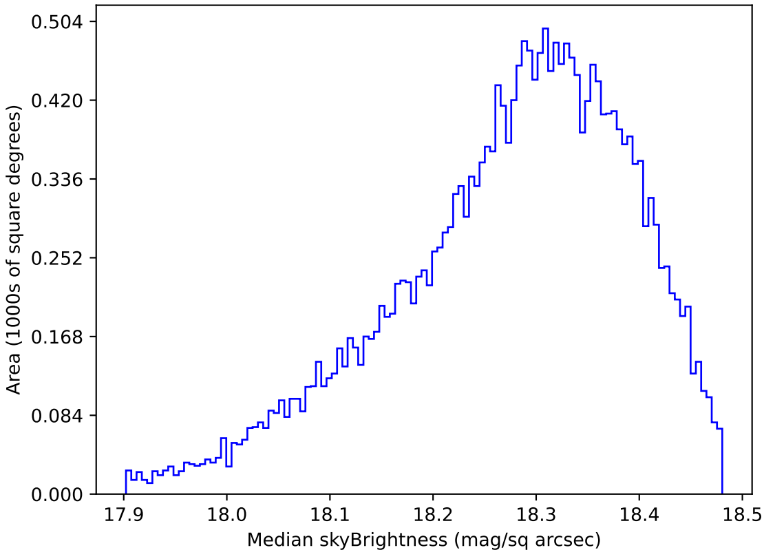
weather_cloudso0v3.4_10yrs Yr 1 y band: Median skyBrightness
