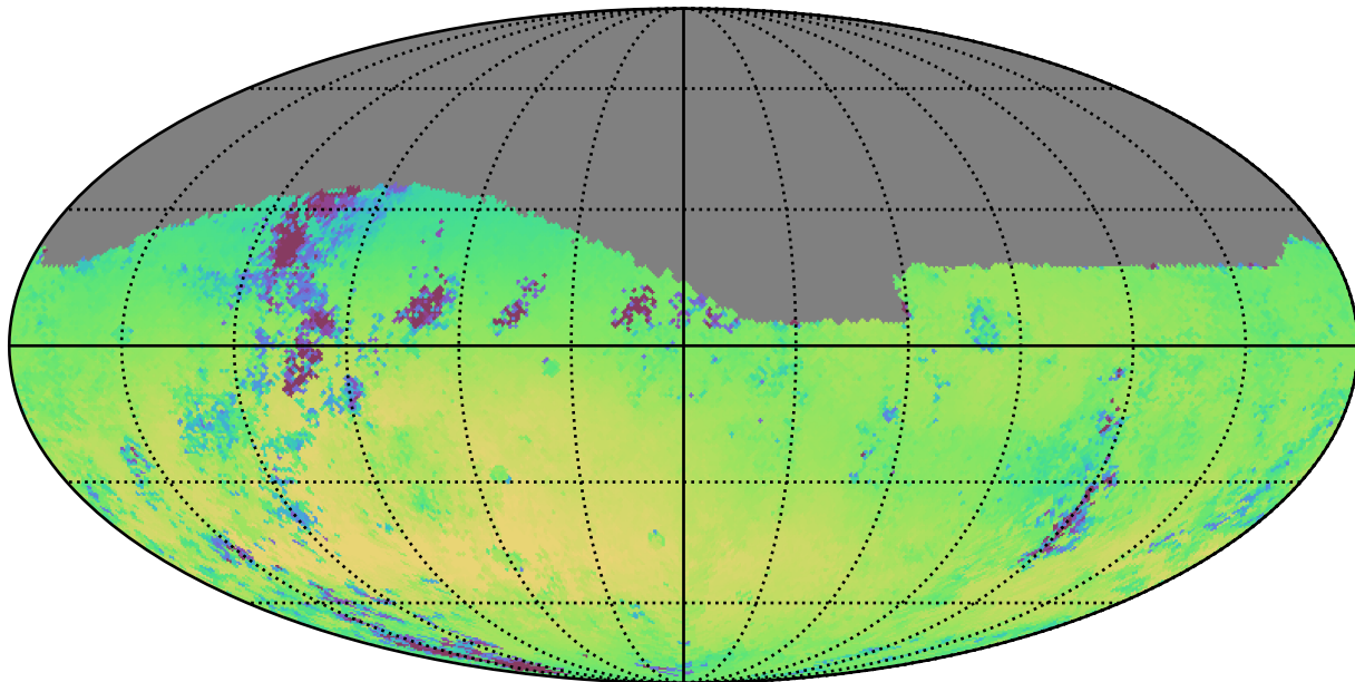
weather_cloudso0v3.4_10yrs Yr 1 r band: Median skyBrightness
