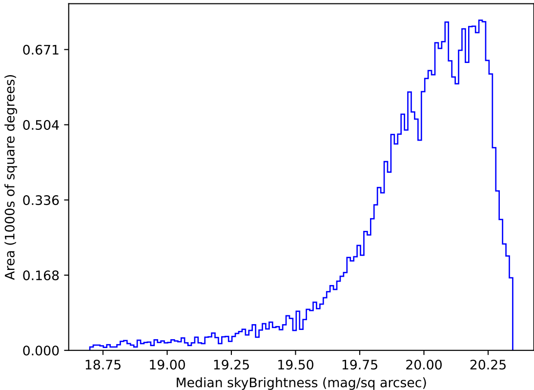
weather_cloudso0v3.4_10yrs Yr 1 i band: Median skyBrightness
