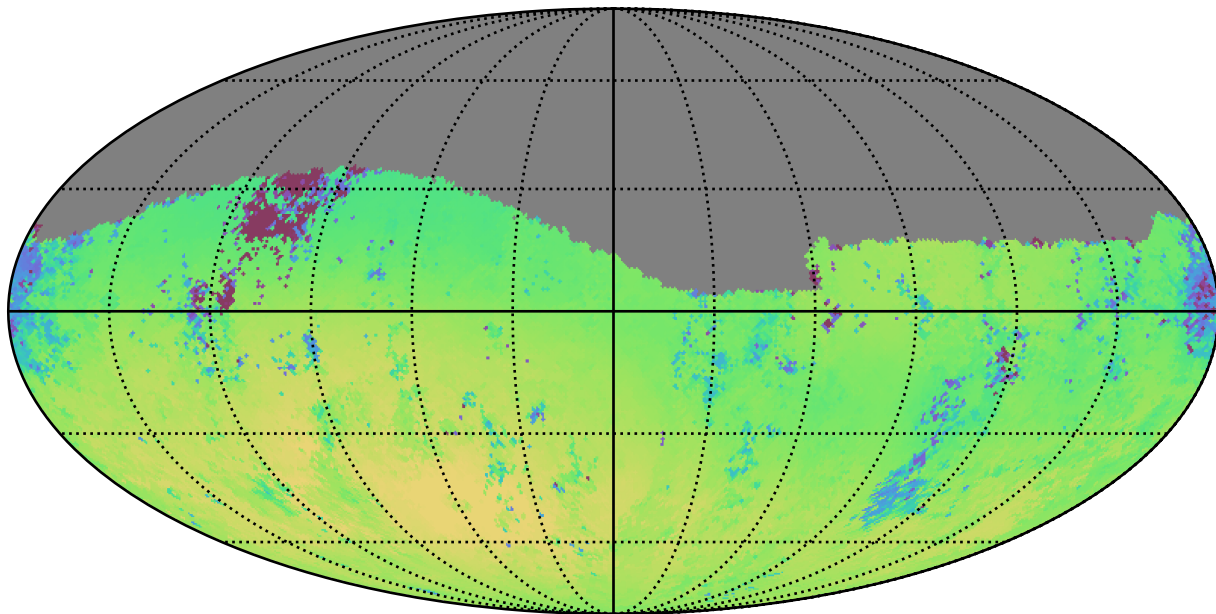
weather_cloudso0v3.4_10yrs Yr 1 g band: Median skyBrightness
