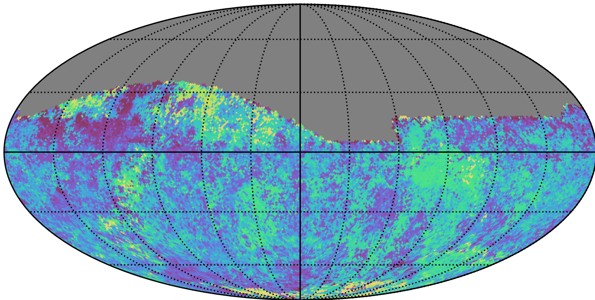
weather_cloudso0v3.4_10yrs Yr 1 all bands: Median skyBrightness
