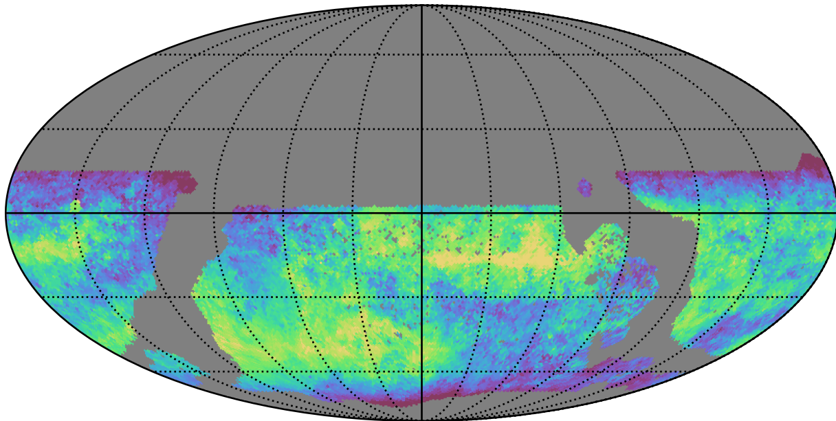
weather_cloudso0v3.4_10yrs WFD z band: Median skyBrightness
