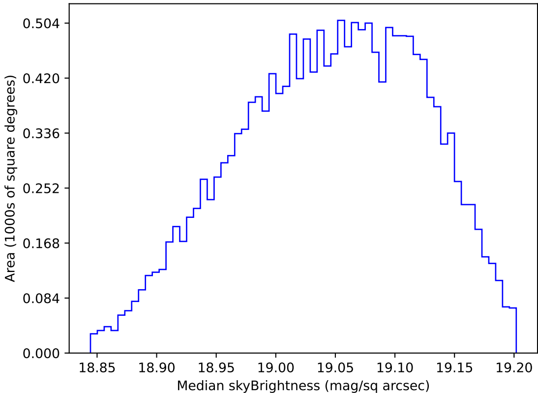
weather_cloudso0v3.4_10yrs WFD z band: Median skyBrightness
