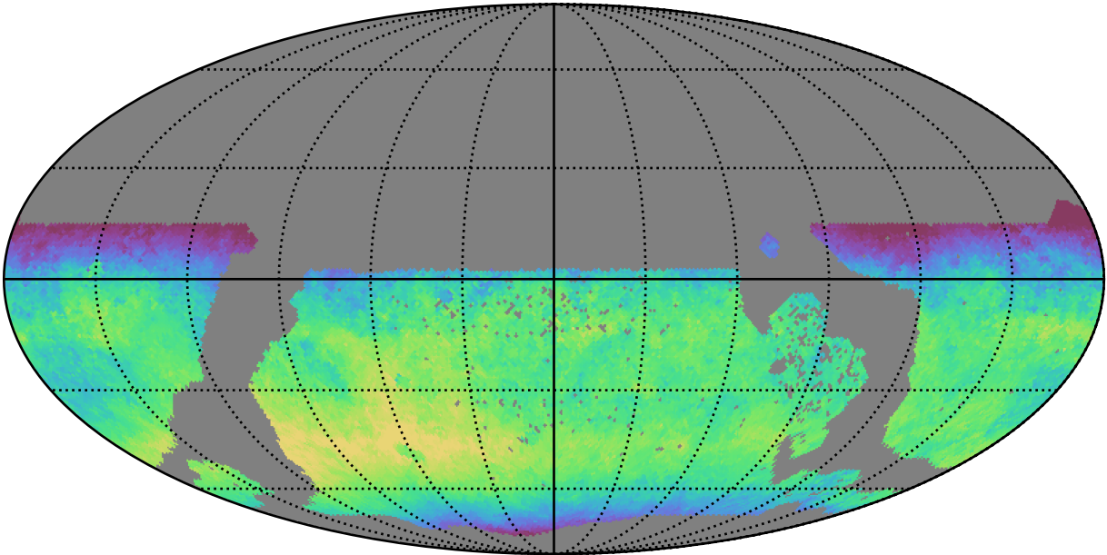
weather_cloudso0v3.4_10yrs WFD y band: Median skyBrightness
