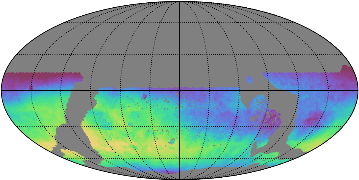
weather_cloudso0v3.4_10yrs WFD u band: Median skyBrightness
