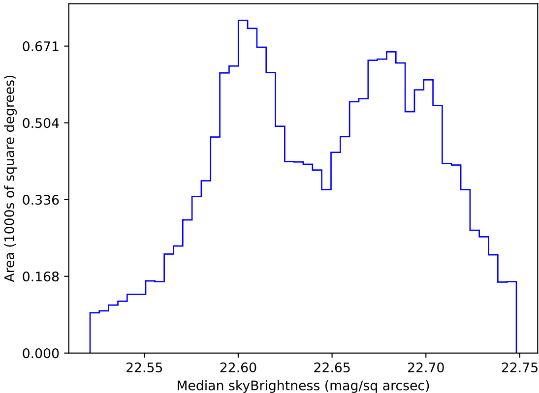
weather_cloudso0v3.4_10yrs WFD u band: Median skyBrightness
